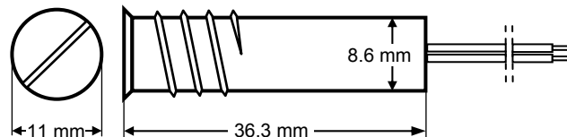
Fig. 3 K-3 reed switch in metal housing
