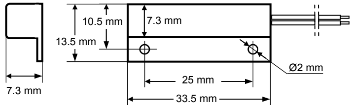
Fig. 1 K-1 reed switch in plastic housing
