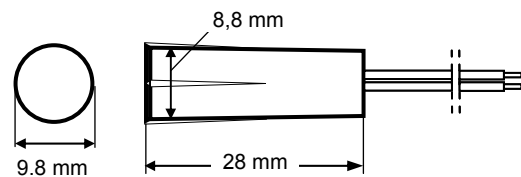
Fig. 2 K-2 reed switch in plastic housing
